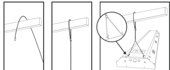
Installation Clips
